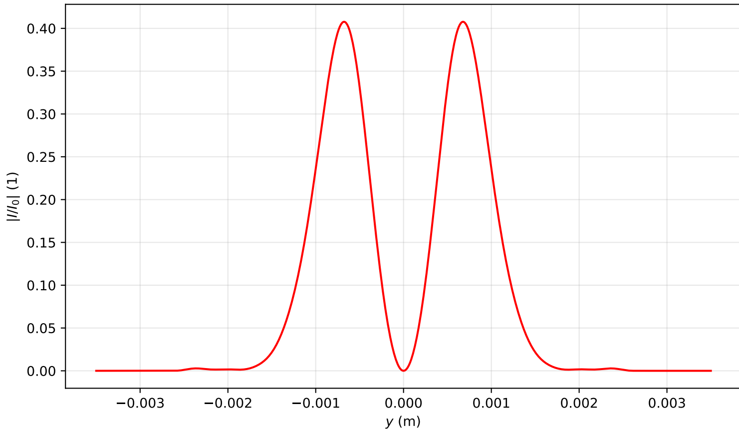
Intensity profile I(x=0, y, z=2.309)/I_0 , P_{in}=3.0P_{cr} , artificial time
